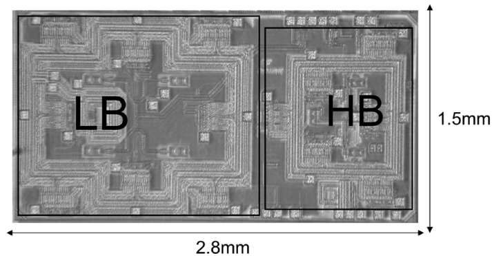
Fig. 18. Die photograph of quad-band fully integrated CMOS PA.
