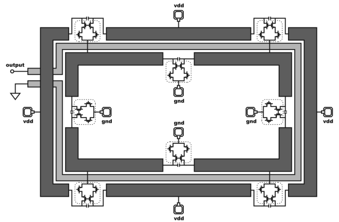
Fig. 8. Double-concentric quad-core DAT with cascode drivers.
