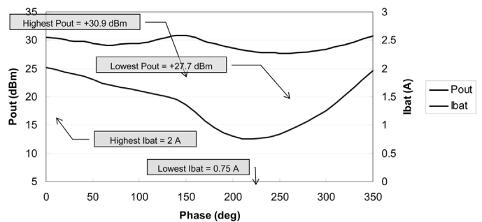
Fig. 17. Output power and the battery current under 4:1 VSWR load mismatch ( \sim 6:1 at the antenna).
