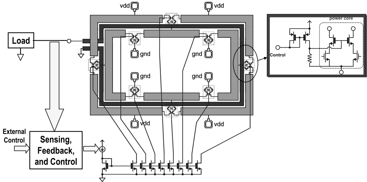
Fig. 9. The distributed power control system.
