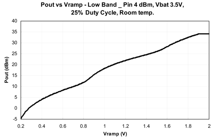
Fig. 16. V_{\text{ramp}} control characteristics.
