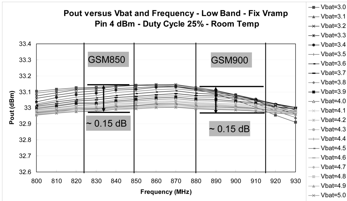
Fig. 13. Power control accuracy for different supply voltages.
